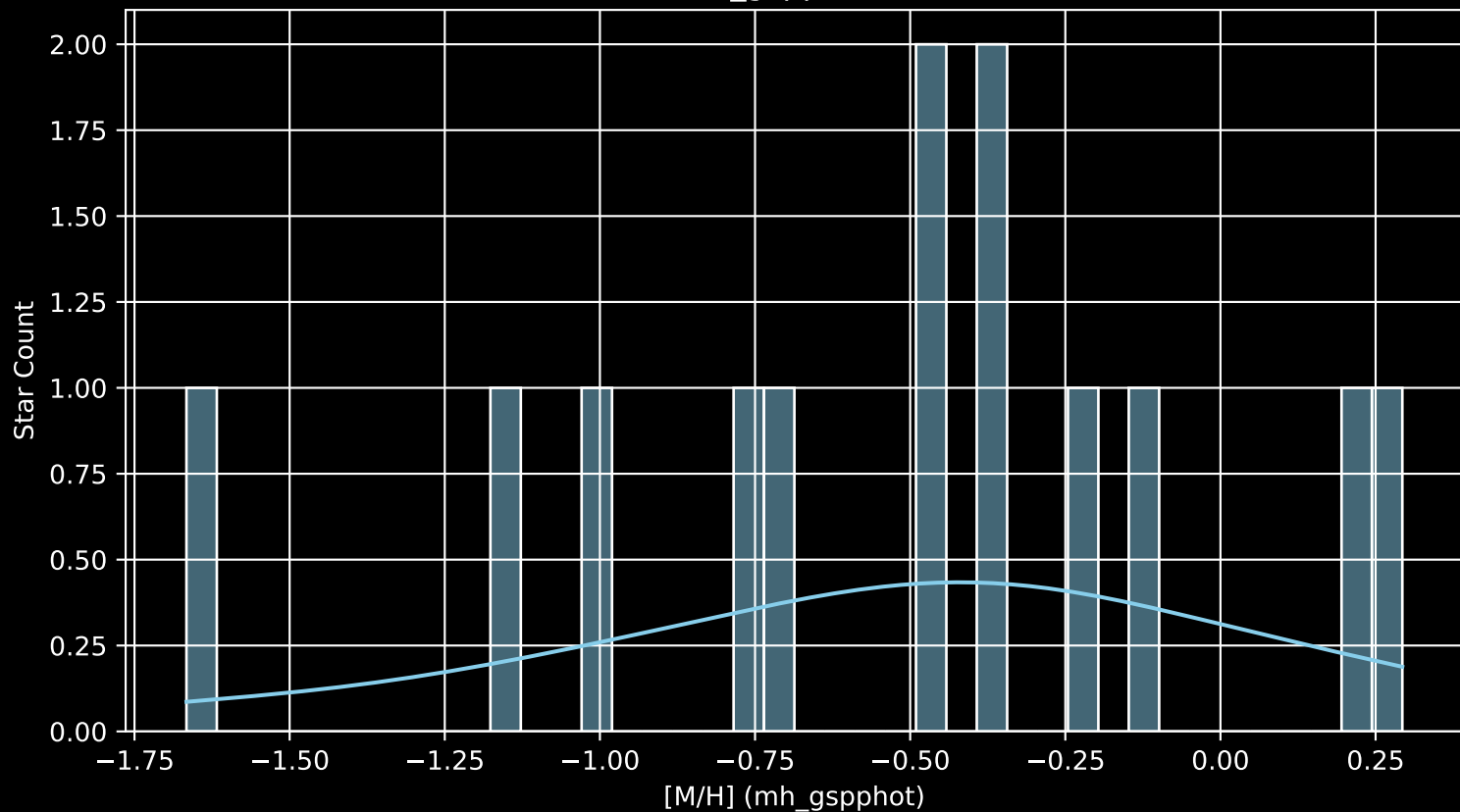
APOGEE DR17 Field: [TESS_OBAF [M/H] (mh_gspphot) (n= 13)
