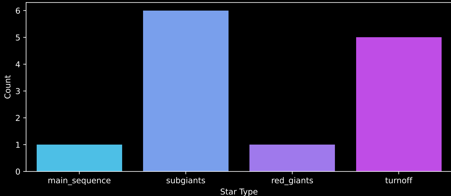
APOGEE DR17 Field: [TESS_OBAF] Count plot of Star Type
