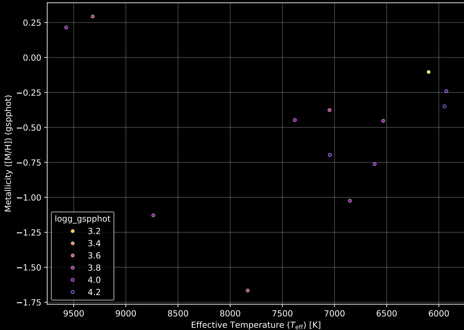
APOGEE DR17 Field: [TESS_OBAF] Stellar Population Parameters (n= 13)
