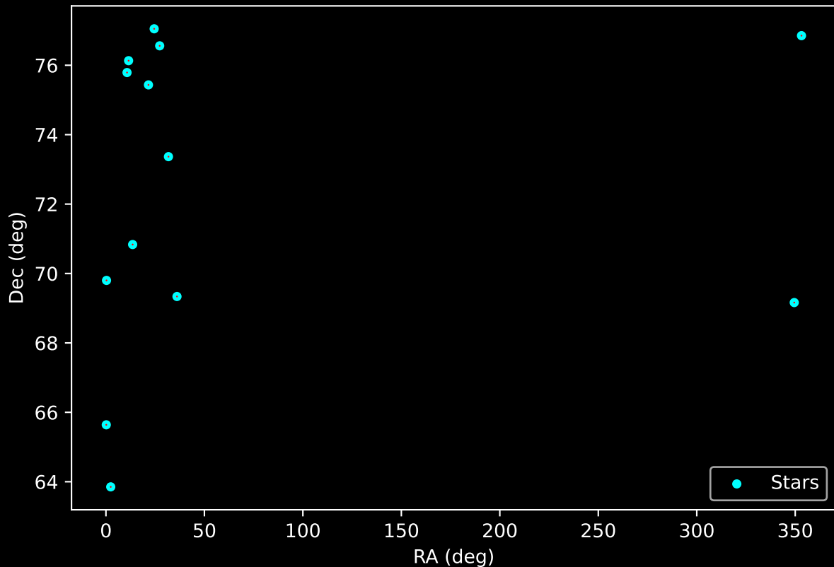
APOGEE DR17 Field: [TESS_OBAF] Proper Motion Vectors for Gaia Star Field (n= 13)
