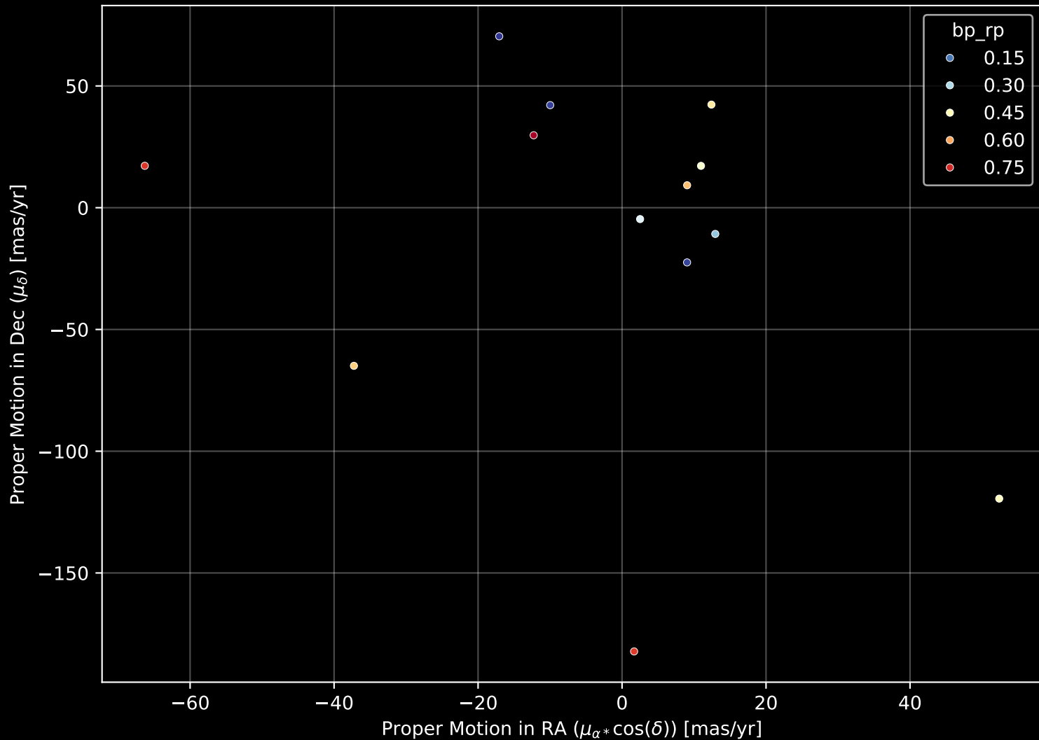
APOGEE DR17 Field: [TESS_OBAF] Proper Motion Diagram (n= 13)
