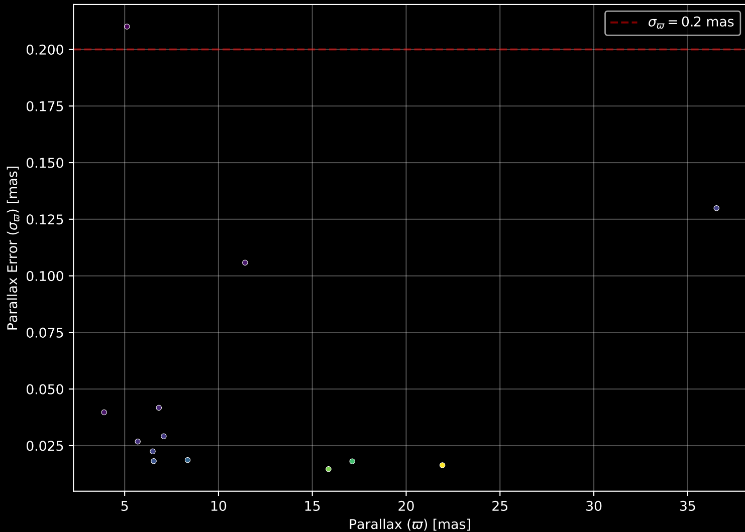
APOGEE DR17 Field: [TESS_OBAF] Parallax Quality (n= 13)
