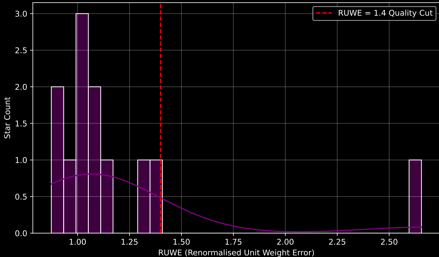
GAPOGEE DR17 Field [TESS_OBAF] RUWE Distribution (n= 12)
